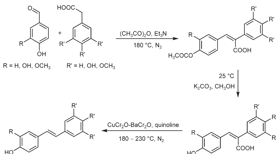
Scheme 1. Synthesis of the the hydroxystilbenes 4–13 .
